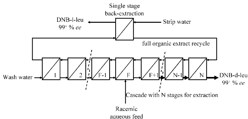
Figure 8. Schematic representation of a countercurrent setup of N CCSs for chiral separation with full recycle of the extract stream
